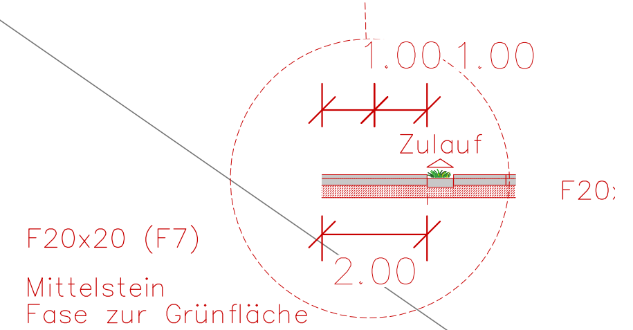
Detail F-Bord
